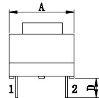
FRONT VIEW (正视图)
