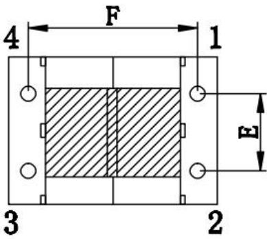
BOTTOM VIEW (底视图)
